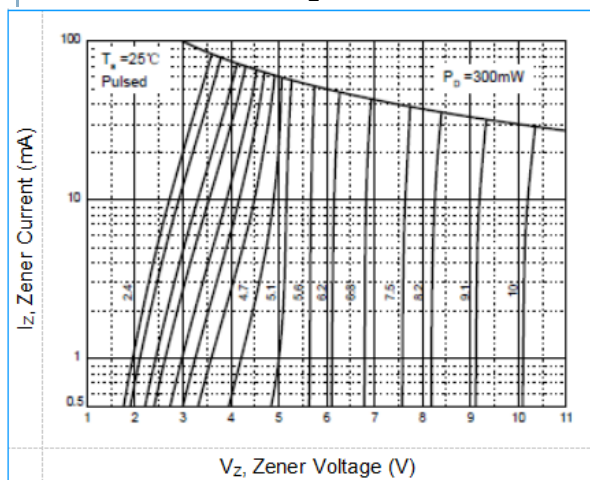
Fig1. Zener Characteristics ( V_Z Up to 10V)
