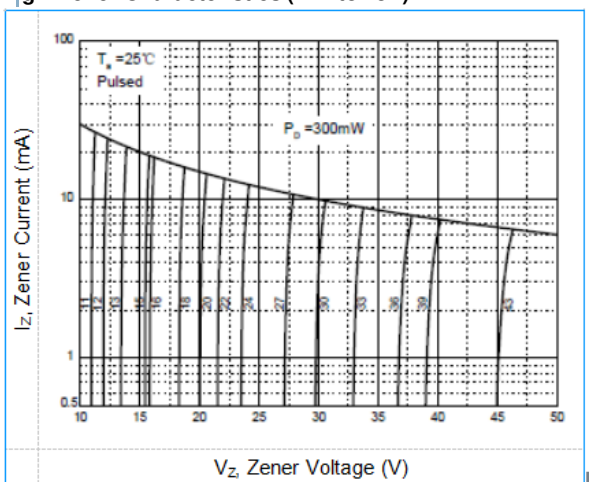
Fig2. Zener Characteristics (11V to 43V)
